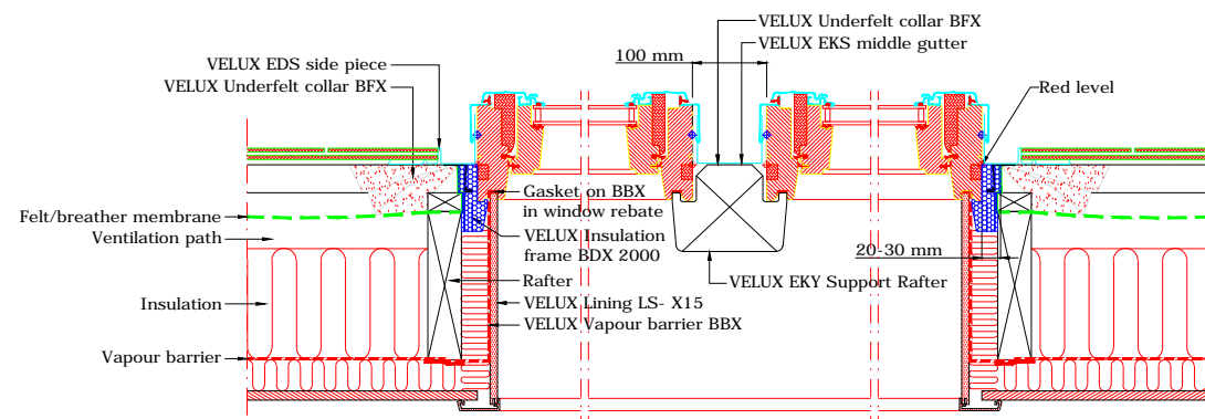
Section B-B 1:10
