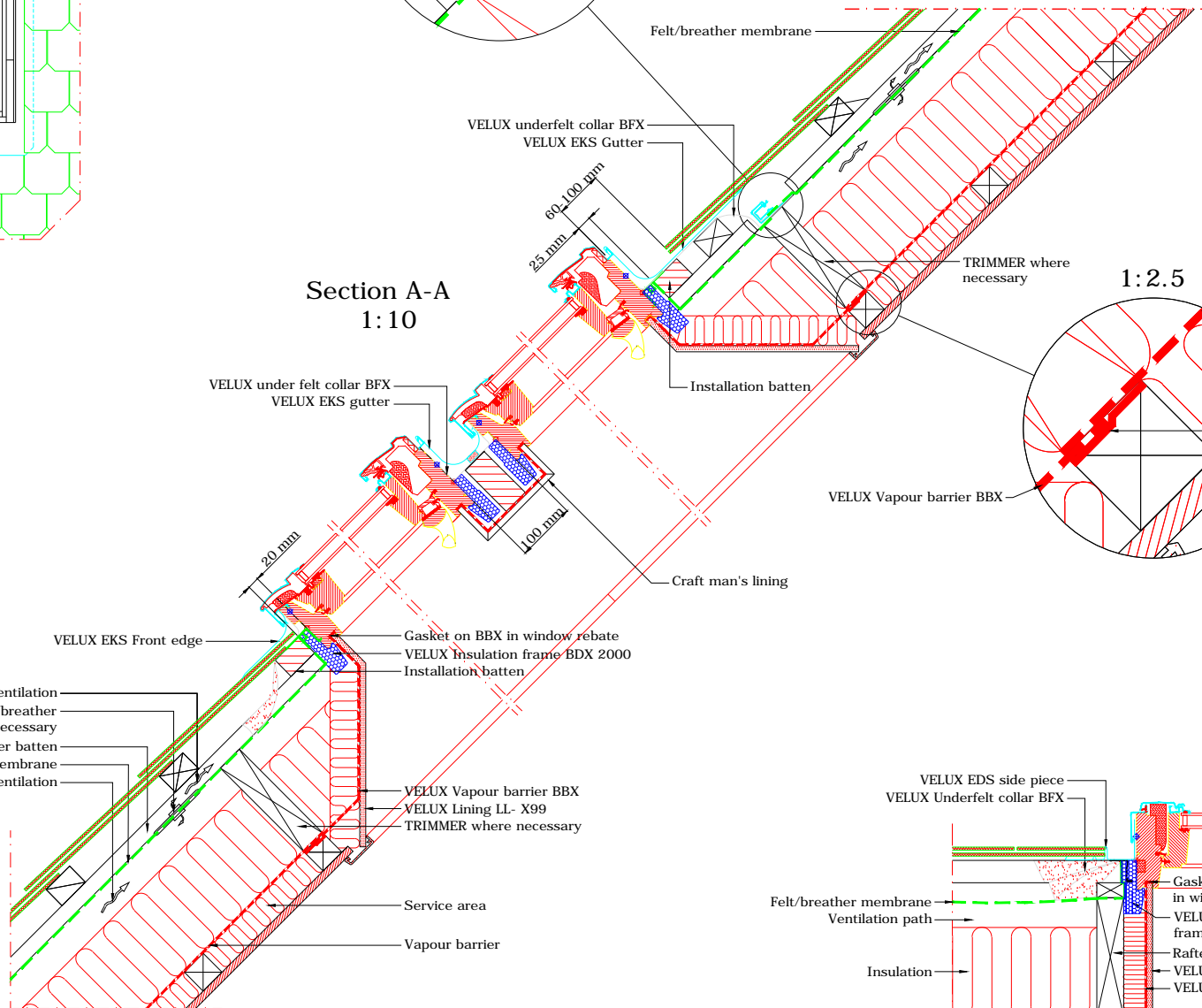
Sheer plan perpendicular to roof
