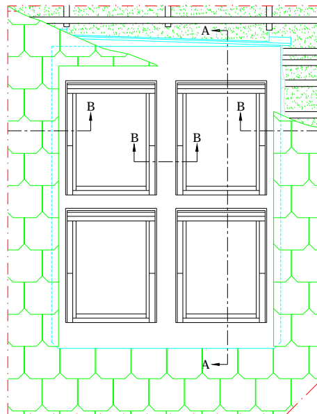
Sheer plan perpendicular to roof
